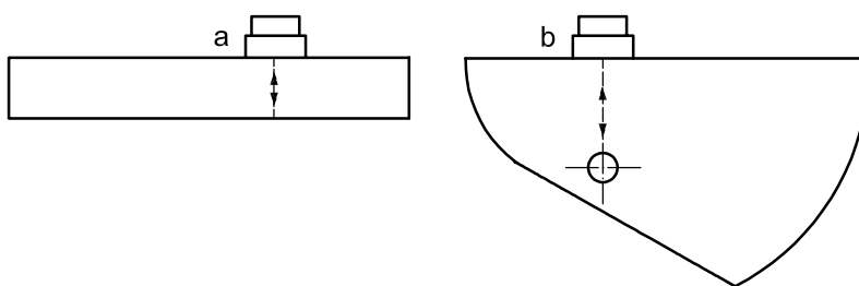
Figure 4 — Straight-beam probes — Sensitivity setting
