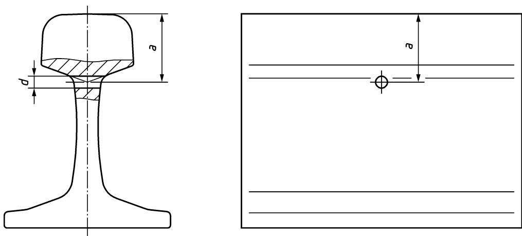
Figure A.14 — Bolt hole slot position D
