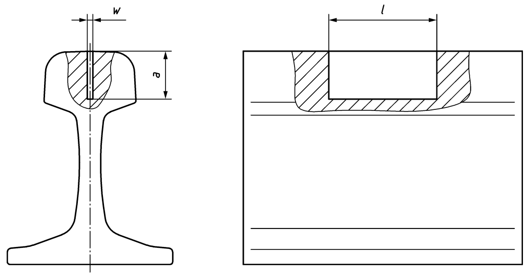
Figure B.4 — Horizontal head-web reflector (rail end)
