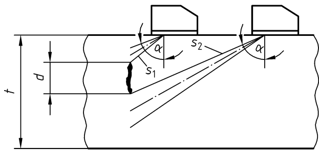
a) Interrupted reflector
