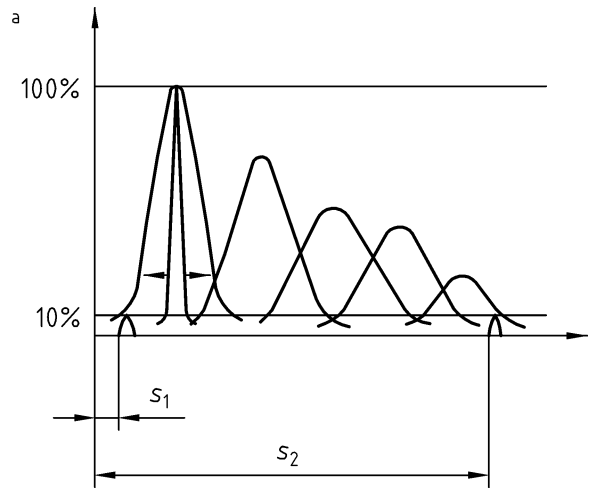
a) Interrupted reflector
