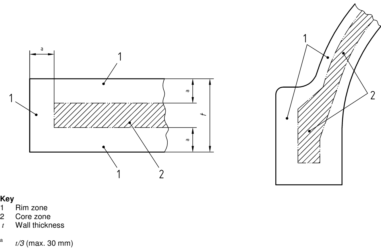
Figure 2 — Division of wall section into zones
