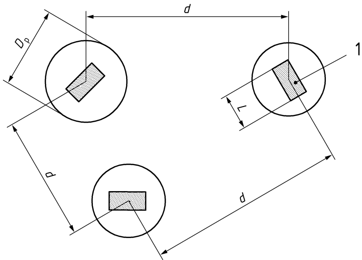
Figure 4 — Extended discontinuity ( L > D_p )
